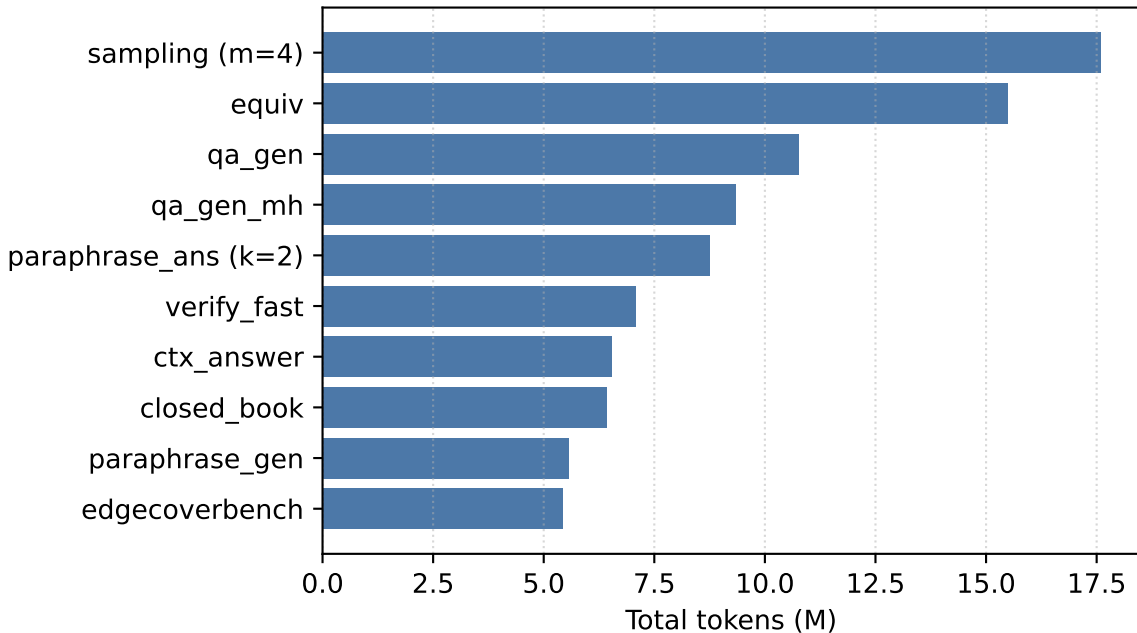
Token breakdown (all call logs)
