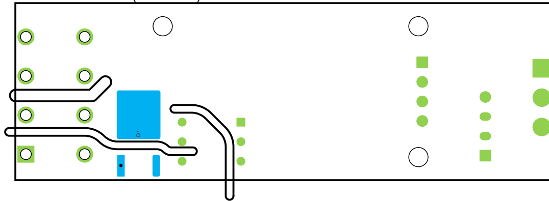
Bottom SMD/THT (Scale 2:1)
