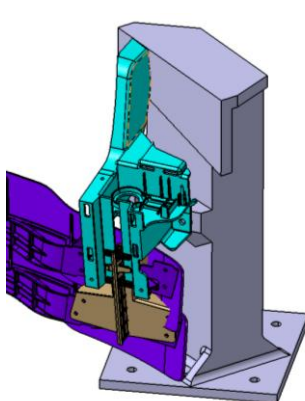
FIXTURE BLOCK
