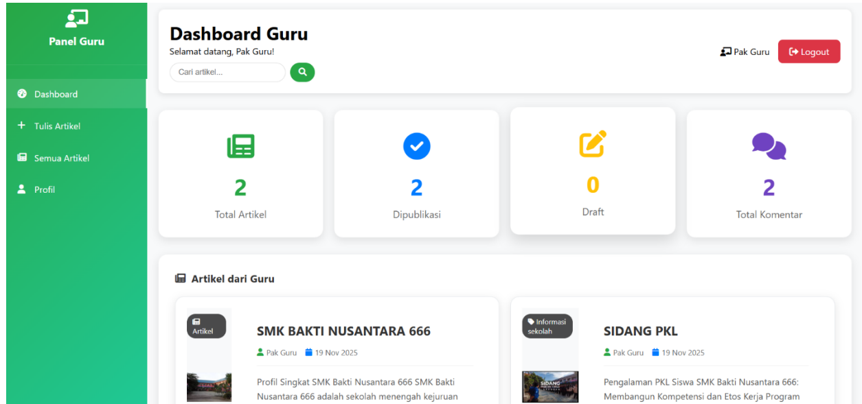
Dasboard Guru
