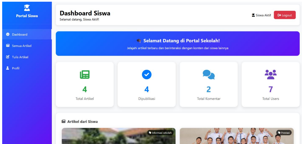
Dashboard Siswa
