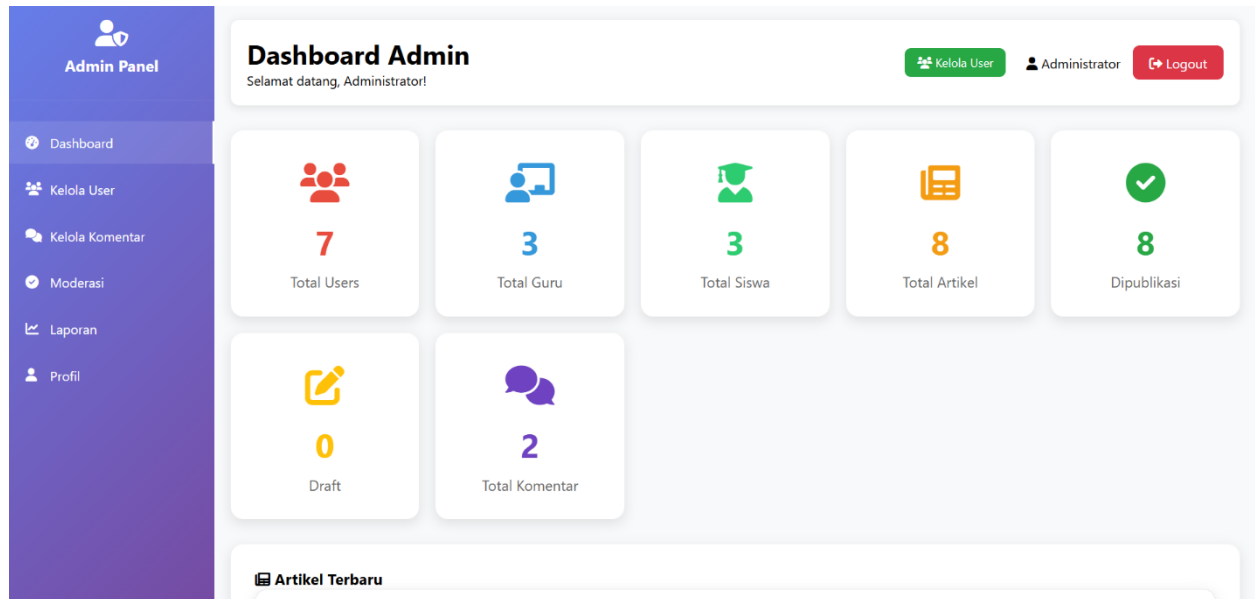
Dashboard Admin
