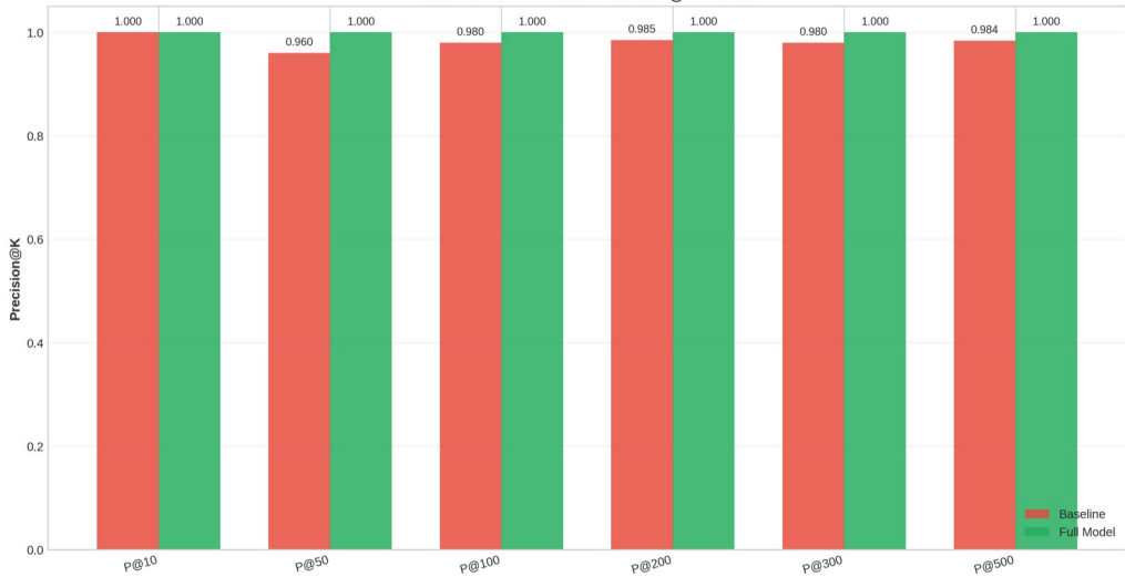
Baseline vs Full Model: Precision@K Metrics
