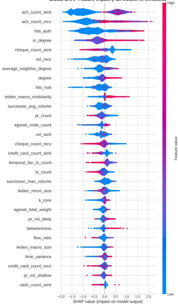
Global SHAP Feature Impact (Full Model, All Windows)
