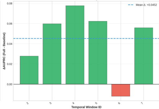
Per-Window AUPRC Improvement
