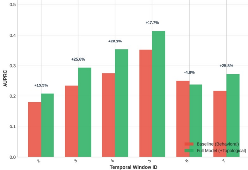
Ablation Study: AUPRC per Temporal Window
