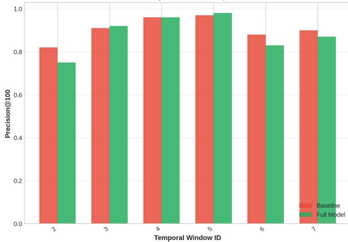
Ablation Study: Precision@100 per Window
