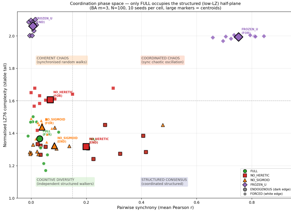
Figure 1: Coordination phase space (\bar{r}, C_{\text{LZ}}) for four ablation conditions under two protocols (BA m = 3 , N = 100 , degree_linear , 10 seeds each). Each point is one run; filled markers are centroids \pm std. Quadrant boundaries: \bar{r} = 0.15 , C_{\text{LZ}} = 1.6 . FULL is the only condition that occupies the structured half-plane ( C_{\text{LZ}} < 1.6 ) in both protocols. FROZEN_U migrates to the chaotic quadrant (high sync, high LZ) under forcing—a signature of coherent chaos . Ablating u ( FROZEN_U ) produces strongly seed-dependent trajectories with high LZ regardless of protocol.
