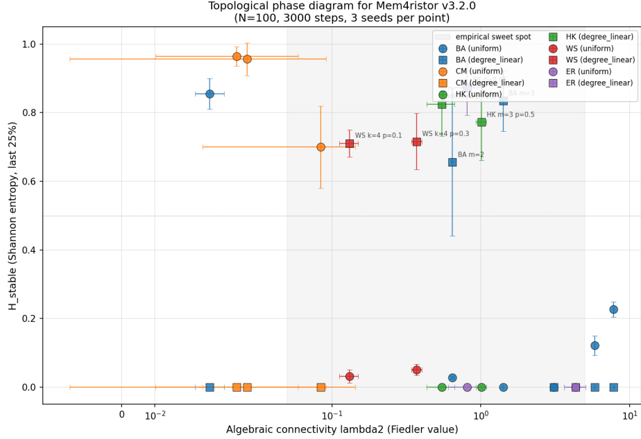
Figure 2: Fiedler phase diagram: algebraic connectivity \lambda_2 vs. cognitive entropy H_{\text{cog}} across diverse network families (Barabási-Albert m \in \{1, 2, 3, 5, 8, 10\} , Configuration Model \gamma \in \{2.5, 3.0, 4.0\} , Holme-Kim, Watts-Strogatz, Erdős-Rényi; N \approx 100 ; two coupling normalizations per topology, n = 30 data points). Complete linear separation between functional (open symbols) and dead-zone (filled symbols) regimes. The regime boundary \lambda_{2,\text{crit}} \in (2.13, 2.50) , midpoint 2.31, is derived from logistic regression on the independent primary dataset ( p2_edge_betweenness.csv , n = 36 ; see text).
