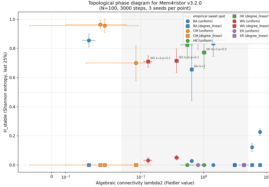
Figure 5: Fiedler phase diagram: algebraic connectivity \lambda_2 vs. cognitive entropy H_{\text{cog}} across diverse network families (Barabási–Albert m \in \{1, 2, 3, 5, 8, 10\} , Configuration Model \gamma \in \{2.5, 3.0, 4.0\} , Holme–Kim, Watts–Strogatz, Erdős–Rényi; N \approx 100 ; two coupling normalizations per topology, n = 30 data points). Complete linear separation between functional (open symbols) and dead-zone (filled symbols) regimes. The regime boundary \lambda_{2,\text{crit}} \in (2.13, 2.50) , midpoint 2.31, is derived from logistic regression on the independent primary dataset ( p2_edge_betweenness.csv , n = 36 ; see text).
