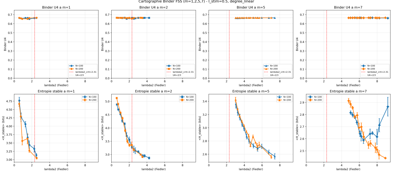
Figure 3: Extended cartography of the Binder cumulant across topologies ( m \in \{1, 2, 5, 7\} , N \in \{100, 200\} , N_{\text{real}} = 701 ). ( Top row ) Binder cumulant U_4 as a function of the algebraic connectivity \lambda_2 for each attachment parameter m . The dashed red line marks the canonical \lambda_{2,\text{crit}} \approx 2.31 , the dotted gray line marks the Gaussian reference U_4 = 2/3 . Across all four topologies and the full \lambda_2 \in [0.5, 10.0] range, U_4 remains within [0.653, 0.667] (amplitude < 0.012 ), with no detectable crossing. This rules out a first-order or two-step Binder transition over the topology range explored. ( Bottom row ) Corresponding order parameter \langle H_{\text{stable}} \rangle . The entropy decreases monotonically with \lambda_2 , with the steepest decline near \lambda_2 \approx 2 for m \in \{1, 2\} and a milder decrease for m \in \{5, 7\} . The combination of a flat U_4 and a monotonic \langle H_{\text{stable}} \rangle is the diagnostic signature of a smooth spectral cross-over, not a thermodynamic phase transition.
