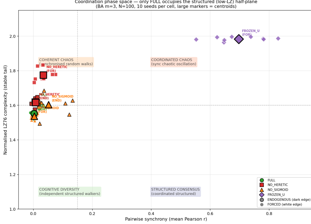
Figure 1: Coordination phase space ( \bar{r}, C_{LZ} ) for four ablation conditions under two protocols (BA m = 3 , N = 100 , degree_linear , 10 seeds each). Each point is one run; filled markers are centroids \pm std. Quadrant boundaries: \bar{r} = 0.15 , C_{LZ} = 1.6 . FULL is the only condition that occupies the structured half-plane ( C_{LZ} < 1.6 ) in both protocols. FROZEN_U migrates to the chaotic quadrant (high sync, high LZ) under forcing—a signature of coherent chaos . Ablating u ( FROZEN_U ) produces strongly seed-dependent trajectories with high LZ regardless of protocol.
