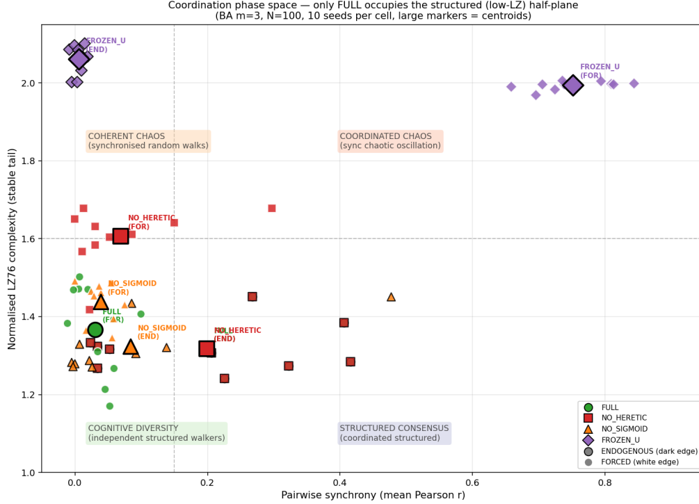
Figure 1: Coordination phase space (\bar{r}, C_{LZ}) for four ablation conditions under two protocols (BA m = 3 , N = 100 , degree_linear , 10 seeds each). Each point is one run; filled markers are centroids \pm std. Quadrant boundaries: \bar{r} = 0.15 , C_{LZ} = 1.6 . FULL is the only condition that occupies the structured half-plane ( C_{LZ} < 1.6 ) in both protocols. FROZEN_U migrates to the chaotic quadrant (high sync, high LZ) under forcing—a signature of coherent chaos . Ablating u ( FROZEN_U ) produces strongly seed-dependent trajectories with high LZ regardless of protocol.
