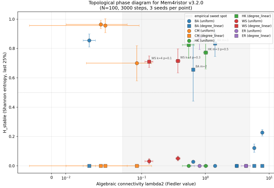
Figure 2: Fiedler phase diagram: algebraic connectivity \lambda_2 vs. cognitive entropy H_{\text{cog}} across diverse network families (Barabási–Albert m \in \{1, 2, 3, 5, 8, 10\} , Configuration Model \gamma \in \{2.5, 3.0, 4.0\} , Holme–Kim, Watts–Strogatz, Erdős–Rényi; N \approx 100 ; two coupling normalizations per topology, n = 30 data points). Complete linear separation between functional (open symbols) and dead-zone (filled symbols) regimes. The regime boundary \lambda_{2,\text{crit}} \in (2.13, 2.50) , midpoint 2.31, is derived from logistic regression on the independent primary dataset ( p2_edge_betweenness.csv , n = 36 ; see text).
