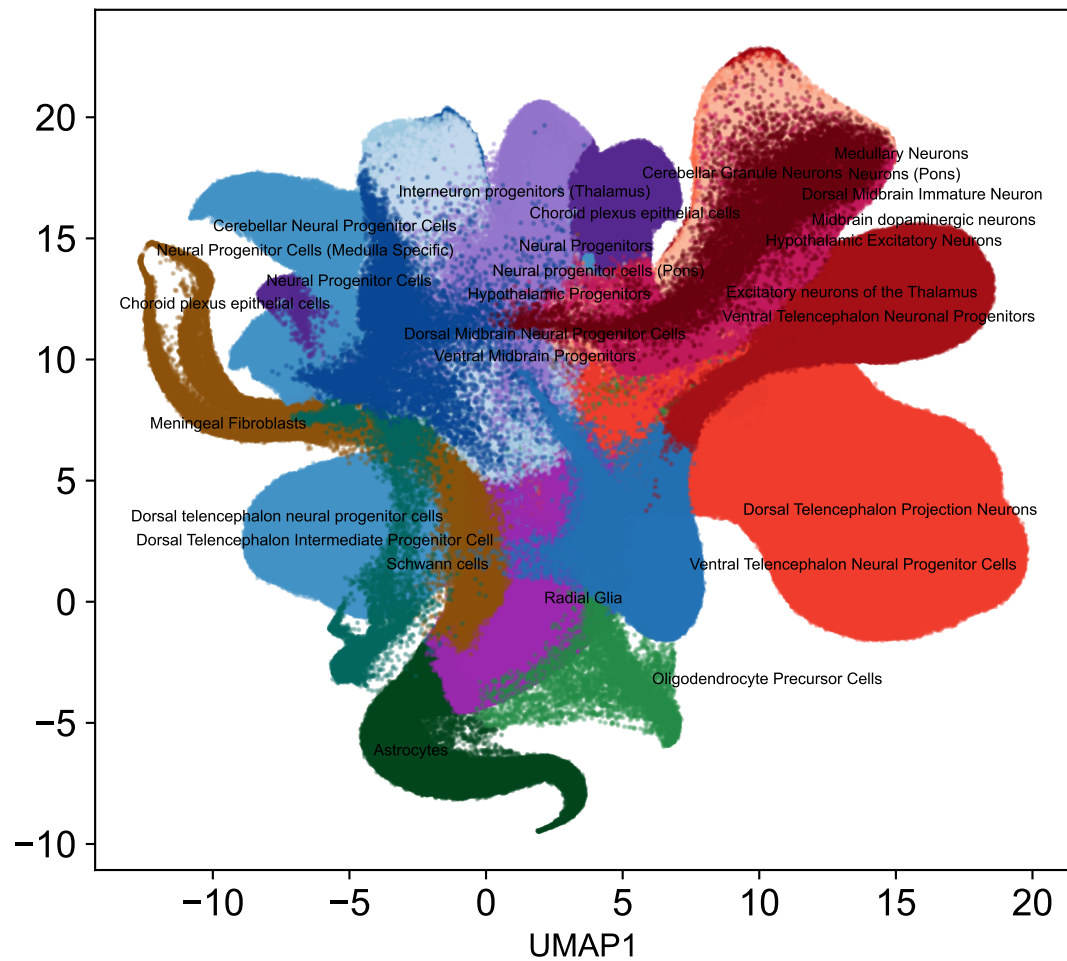
Reference
