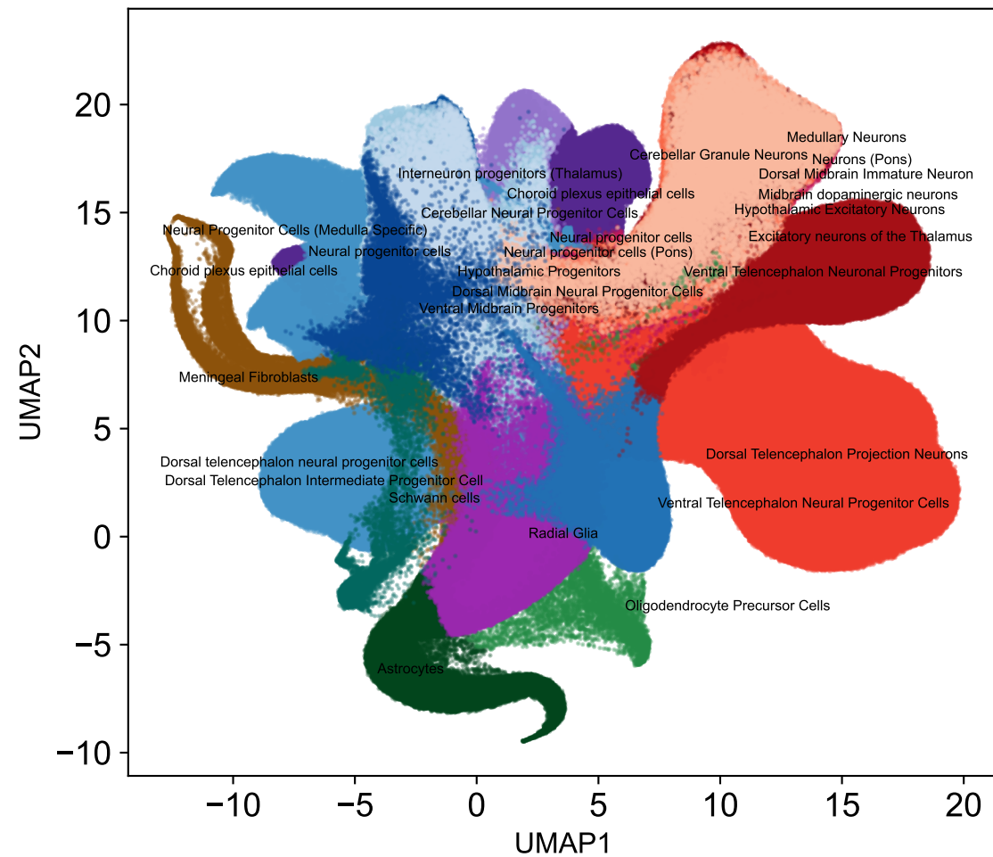
Our Framework
