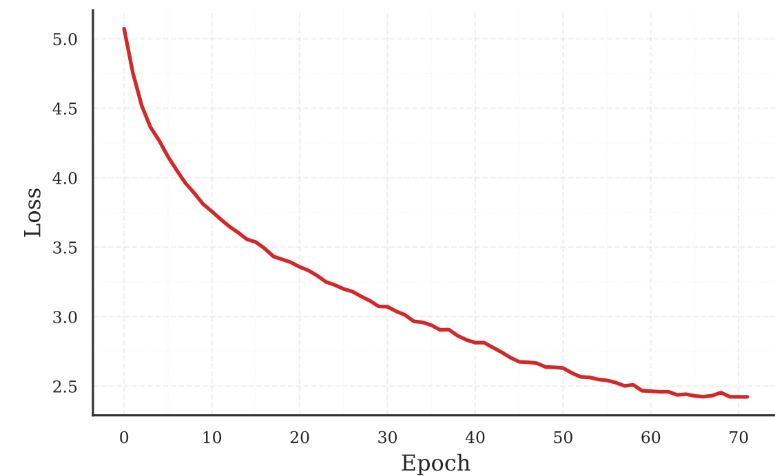
Classification Loss
