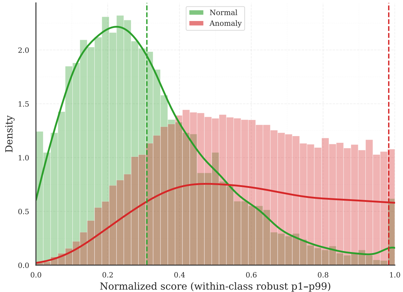
(b) Mahalanobis Distance Distribution
