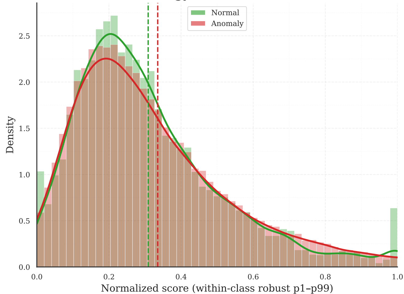
(a) Energy Score Distribution
