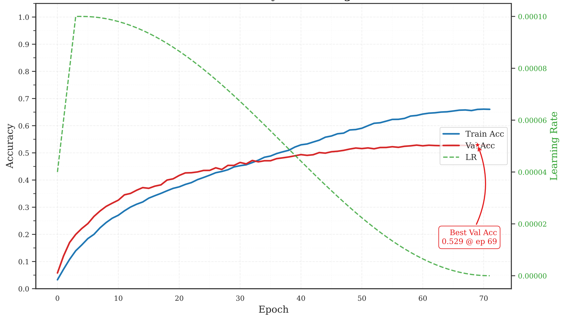
SELYNE: Accuracy & Learning Rate
