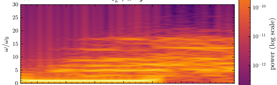
(c) I_L^{S_\alpha}, \alpha = z
