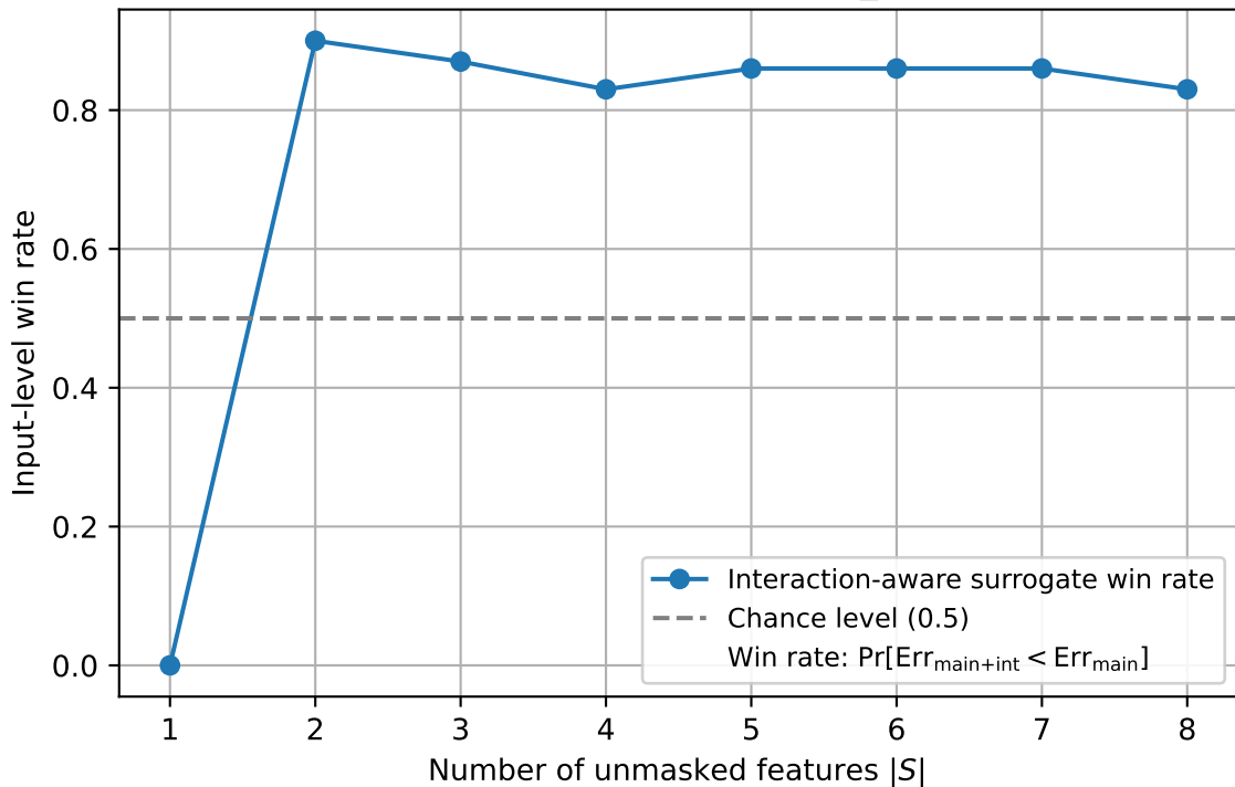
Win rate across inputs — zero_baseline
