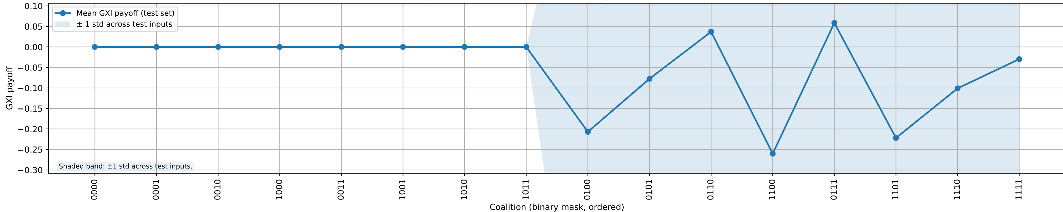
GXI coalition path (test-set mean \pm 1 std) of the game defined on feature i = 1
