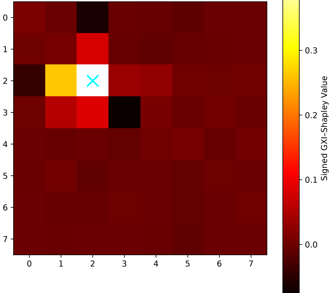
Heat Map of GXI-Shapley Values for Selected Superspixel 18
