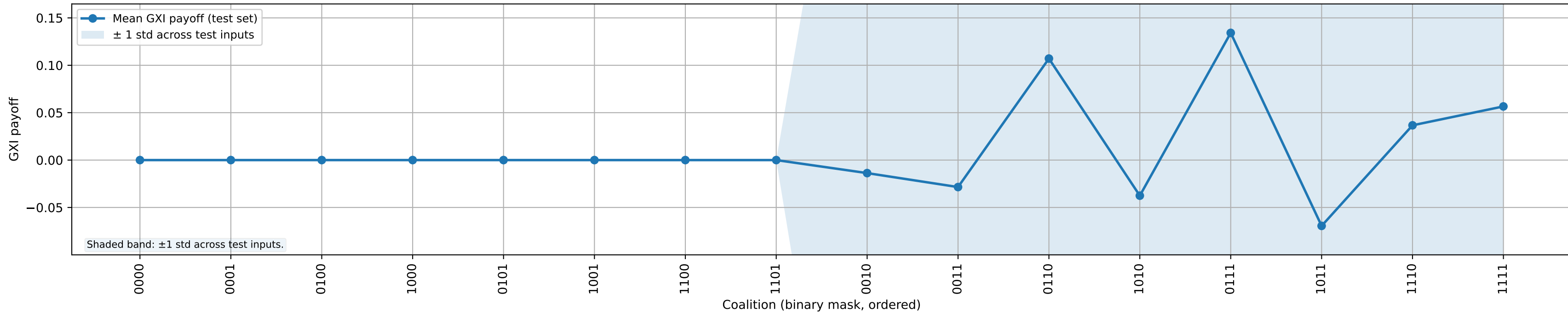
GXI coalition path (test-set mean \pm 1 std) of the game defined on feature i = 2
