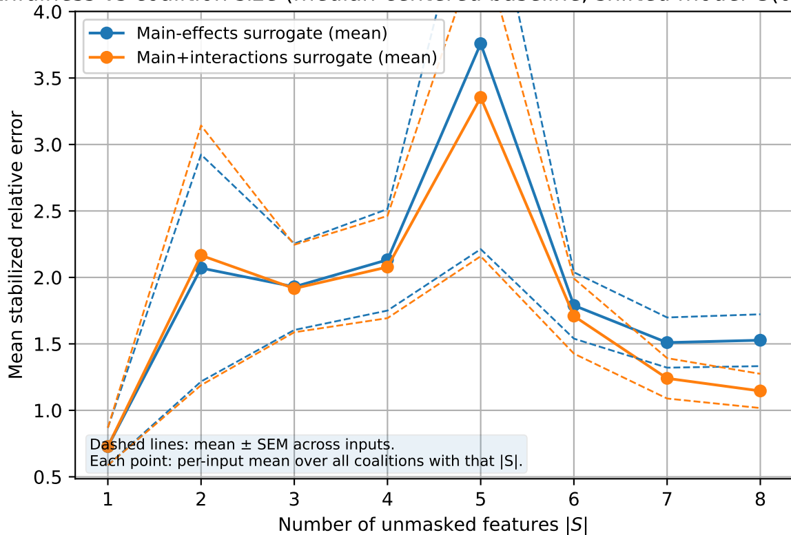
Faithfulness vs coalition size (median-centered baseline, shifted model G(\delta)=F(b+\delta) )
