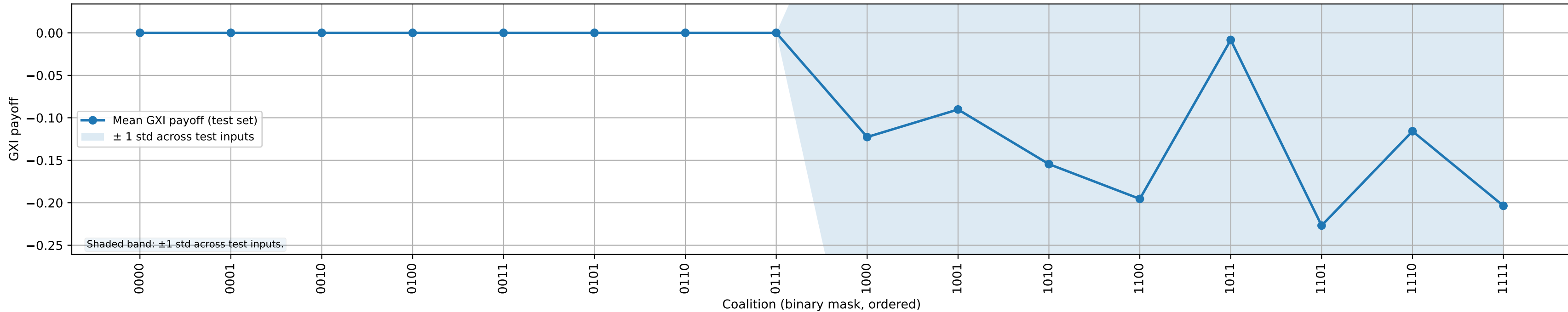
GXI coalition path (test-set mean \pm 1 std) of the game defined on feature i = 0
