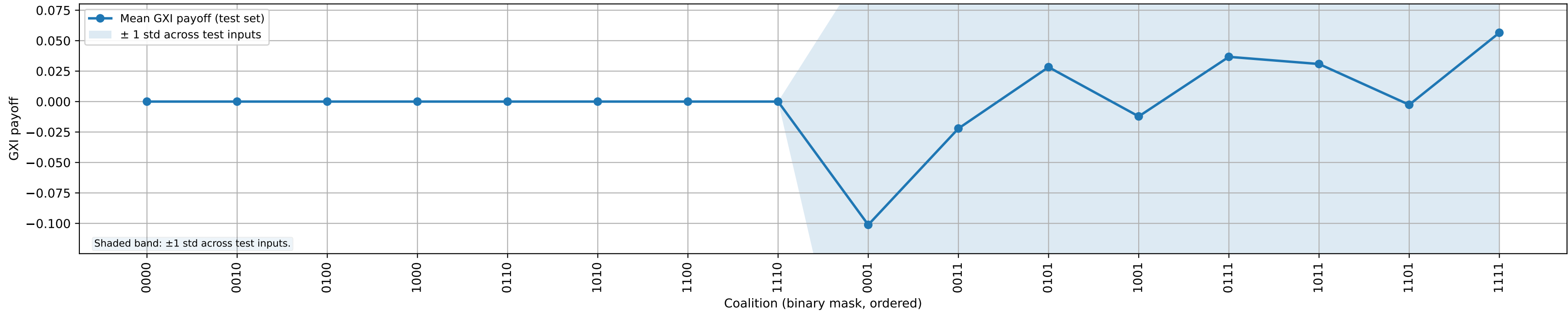
GXI coalition path (test-set mean \pm 1 std) of the game defined on feature i = 3
