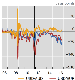
Figure: CIP Deviations (left: 3-month basis; right: 3-year basis)
