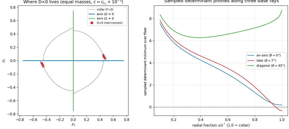
FIGURE 2. Left: sampled negative determinant values near the base collar, with the coordinate axes z_2 = 0 and z_1 = 0 . Right: sampled approximations to D_{\min} along three selected rays. These are base-slice profiles, not computed retrograde or direct trajectories. Floating-point, equal masses, c = c_{L_1} + 10^{-3} .
