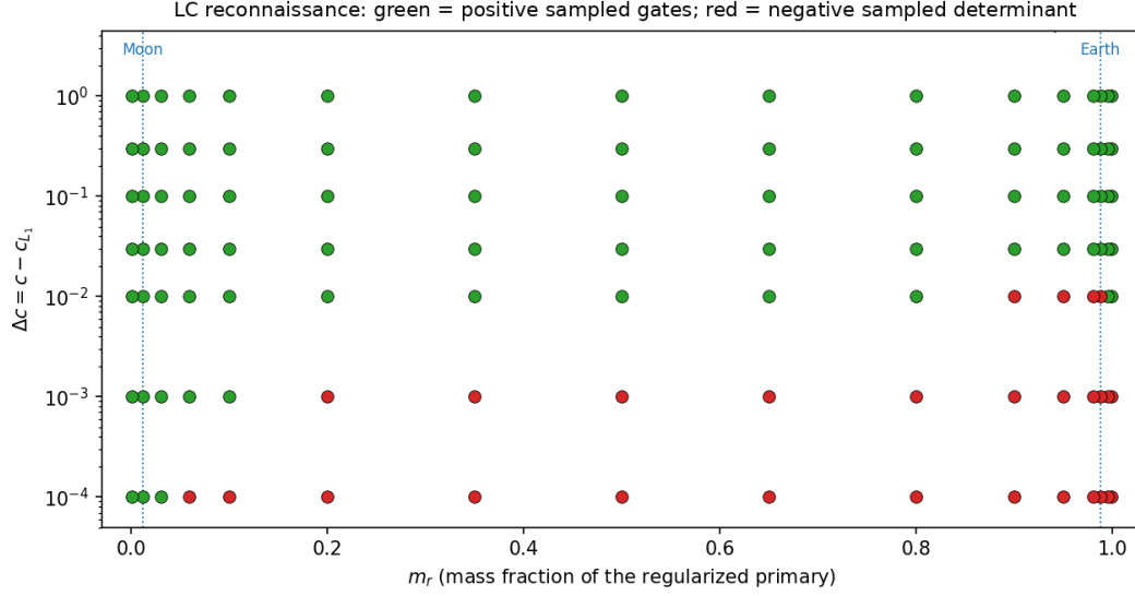
FIGURE 1. Floating-point reconnaissance of LC-convexity in the regularized-primary fraction m_r (Remark 2.1). Green markers: no negative gate value detected by the sampling procedure. Red markers: a sampled determinant value is negative. The Earth and Moon fractions are indicated. These classifications are not interval certificates. No threshold from the Euler problem is asserted for this rotating-model plot; see Section 5.3. The Moon component’s smaller near-critical offsets are examined in Section 5.5.
