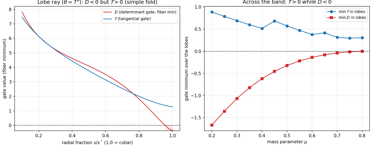
FIGURE 3. Fine structure of the lobes (floating-point, c = c_{L_1} + 10^{-3} ). Left: along a sampled lobe ray ( \theta = 7^\circ , equal masses), the approximation to D_{\min} dips below zero near the collar while the sampled \mathcal{T} stays positive. Right: over the sampled mass values and lobe points, the computed minimum of \mathcal{T} is positive and that of D_{\min} is negative. The labels D in this plot refer to sampled fiber-minimum values, not to the rigorous bound \mathcal{D} .
