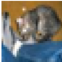
clean: cat (70%)
