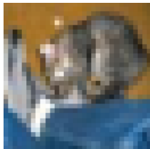
clean: cat (38%)
