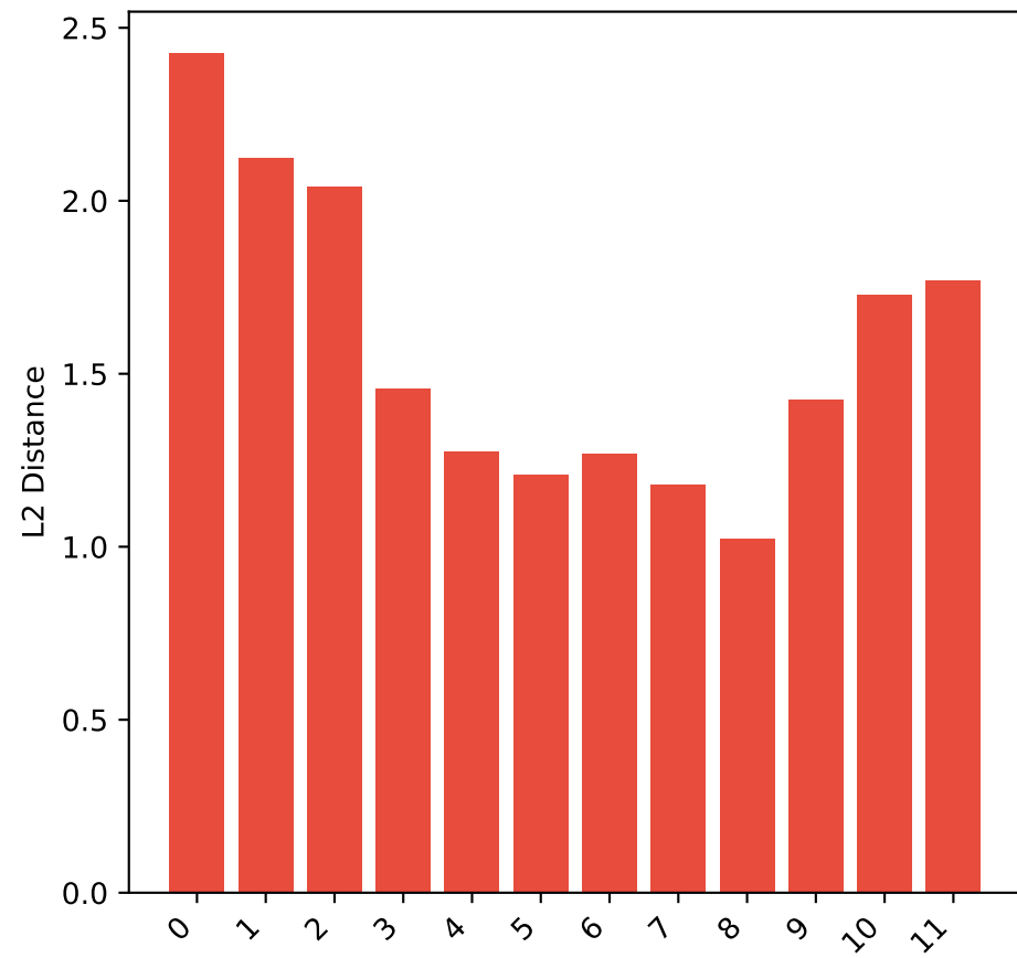
Feature L2 Distance (Clean vs Adversarial) - Run2
