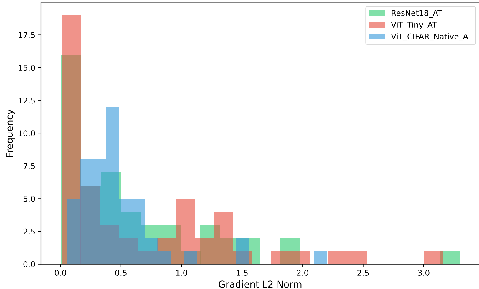
Gradient Norm Distribution: CNN vs ViT
