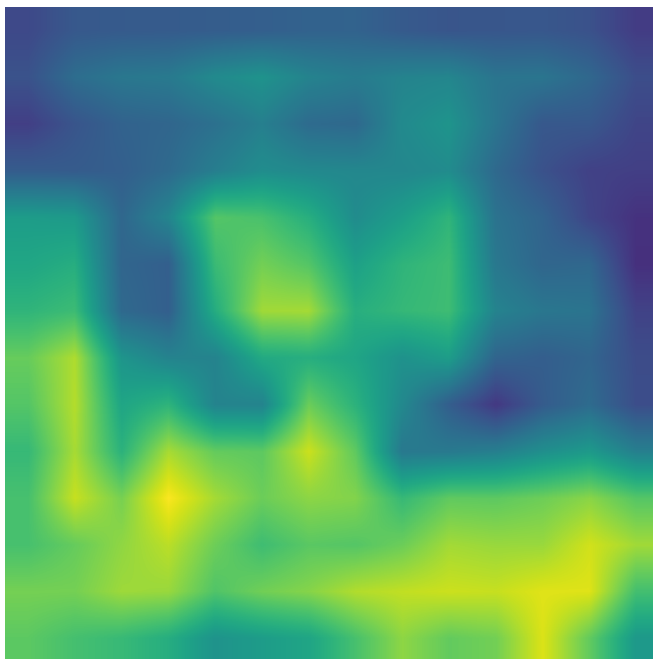
Layer 6 Adversarial
