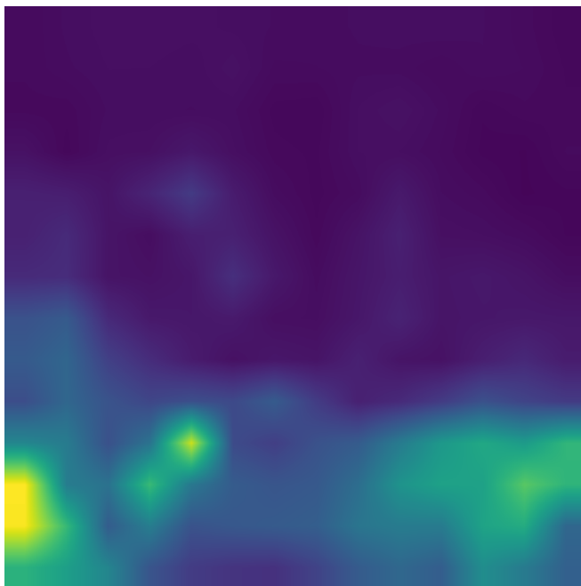
Layer 12 Adversarial
