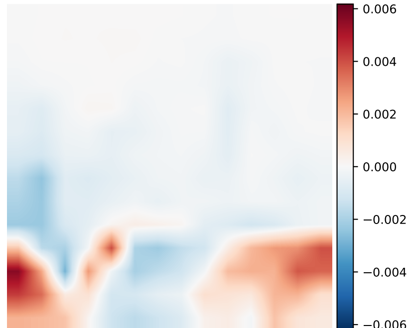
Layer 12 Difference
