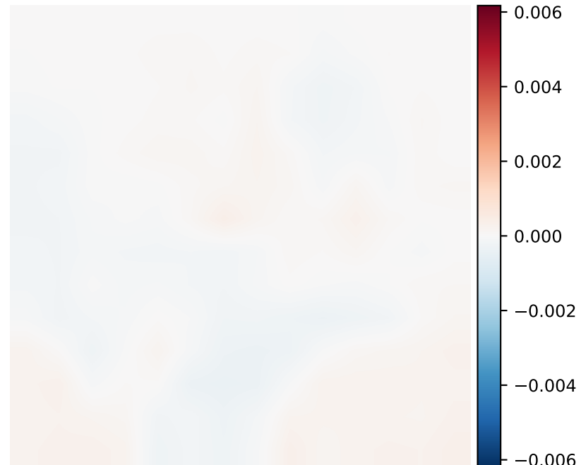
Layer 6 Difference
