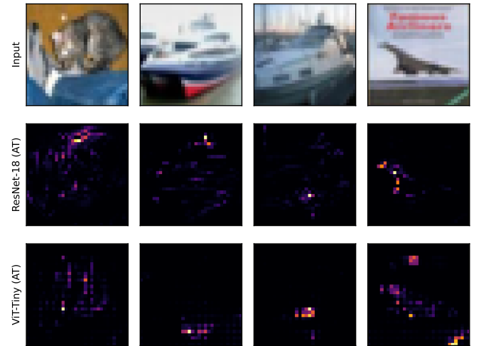
Fig. 6: Input-gradient magnitude maps for the same test images under both models. CNN gradients place more of their mass on fewer components (Table VIII); Table IX shows that this is not accompanied by a difference in spatial arrangement, so the panels should be read as sparsity rather than as localization.
