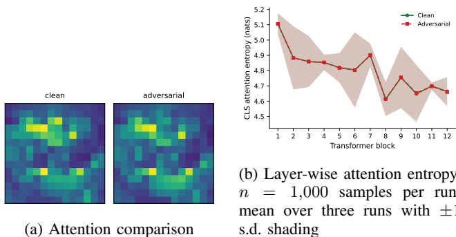
Fig. 8: ViT attention analysis under attack: (a) clean vs. adversarial CLS attention for a representative sample; (b) per-layer entropy of the CLS attention distribution for clean and adversarial inputs.
