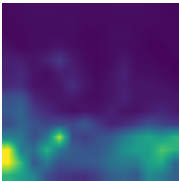
Layer 12 Adversarial
