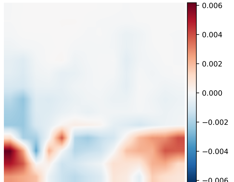
Layer 12 Difference
