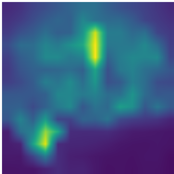
Layer 12 Adversarial
