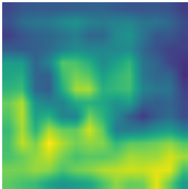
Layer 6 Adversarial
