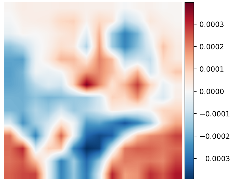
Layer 6 Difference
