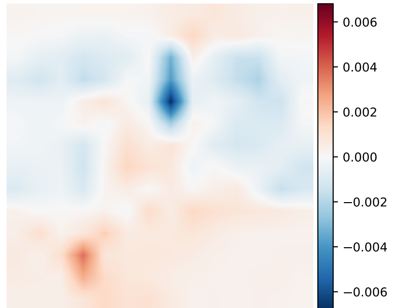
Layer 12 Difference
