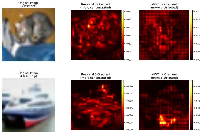
Hoyer sparsity (scale-invariant): ResNet-18 0.474 | ViT-Tiny 0.449
