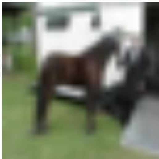
Clean horse (74.0%)
