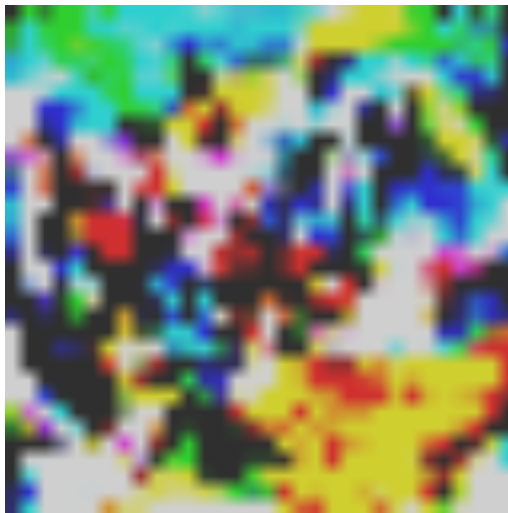
Perturbation ( \times 10 )
