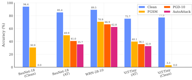
Fig. 1: Clean, FGSM, PGD-10, and AutoAttack accuracy at \epsilon = 8/255 on the full CIFAR-10 test set. CNNs outperform ViTs under standard adversarial training; WideResNet-28-10 achieves the highest robust accuracy through capacity, additional training data, and a stronger recipe jointly [48] (its AutoAttack bar is the RobustBench-reported value).
