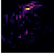
ResNet-18 (AT)
