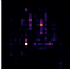
ViT-Tiny (AT)
