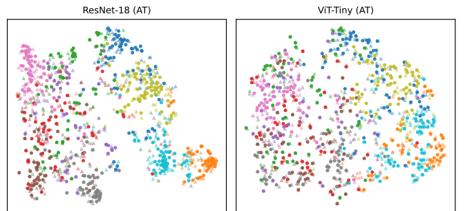
Fig. 9: Illustrative t-SNE embedding of penultimate features for clean samples (circles) and white-box PGD-10 adversarial samples (triangles), for ResNet-18 (left) and ViT-Tiny (right). t-SNE is shown for orientation only; the quantitative comparison is given in the text.
