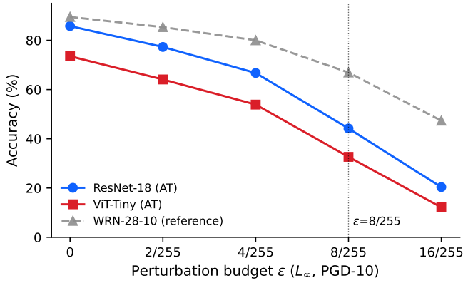
Fig. 2: PGD-10 robust accuracy vs. perturbation budget ( \epsilon ), measured on the full test set. Both AT architectures degrade with similar shapes as epsilon increases, with the CNN maintaining a consistent margin.
