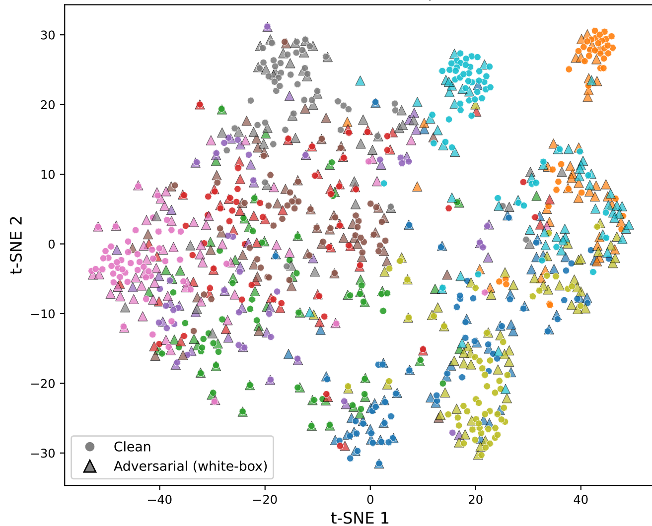
ResNet-18 Feature Space
