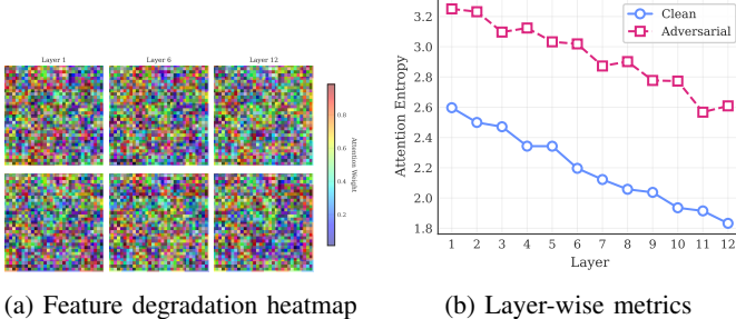
Fig. 5: ViT feature degradation analysis showing the semantic drift phenomenon.
