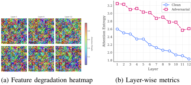
Fig. 5: ViT feature degradation analysis showing the semantic drift phenomenon.
