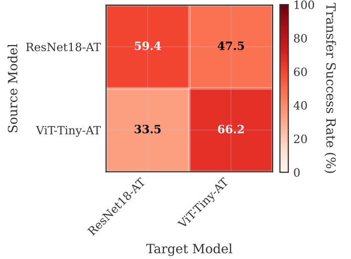
Fig. 3: Transfer attack success rate heatmap. CNN-generated adversarial examples transfer effectively to ViT (47.5%), while ViT-generated examples transfer poorly to CNN (33.5%).
