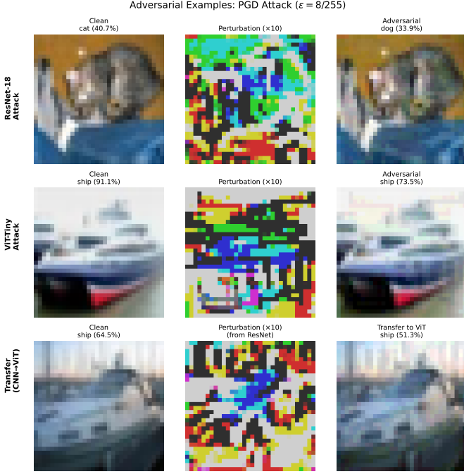
Fig. 2: Adversarial example visualization. Each row shows: original image with model prediction, perturbation magnified 10\times , and adversarial image with new prediction. Row 1: Attack on ResNet-18. Row 2: Attack on ViT-Tiny. Row 3: Transfer attack (generated on ResNet, evaluated on ViT). The perturbations are imperceptible yet cause confident misclassifications.
