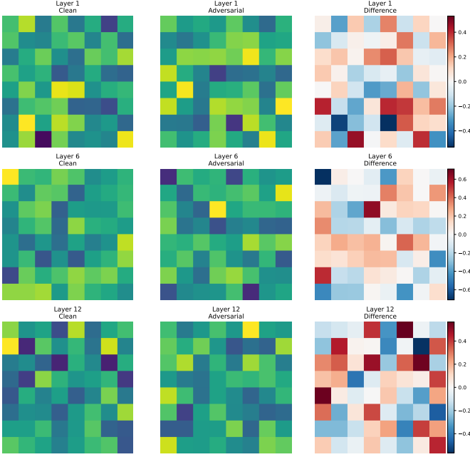
Fig. 7: Attention map comparison across ViT layers under adversarial attack. Each row shows a different layer (1, 6, 12). Columns show clean attention, adversarial attention, and their difference. Early layers maintain similar attention patterns, while late layers show significant attention degradation.
