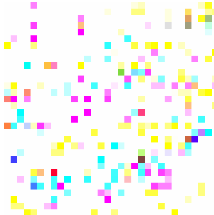
Perturbation (amplified)
