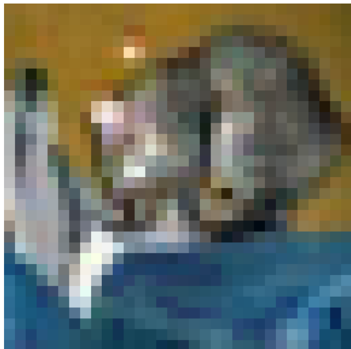
Perturbation (amplified)
