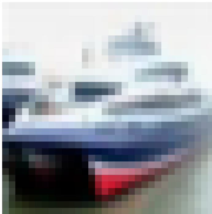
Adversarial (pred: 8)
