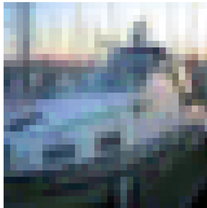
Perturbation (amplified)
