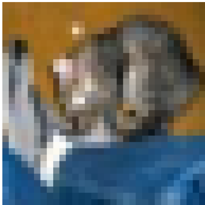
Adversarial (pred: 3)
