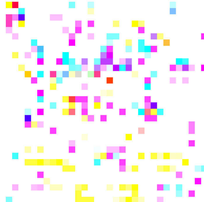
Perturbation (amplified)
