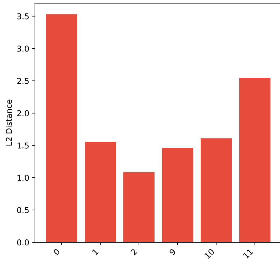
Feature L2 Distance (Clean vs Adversarial)
