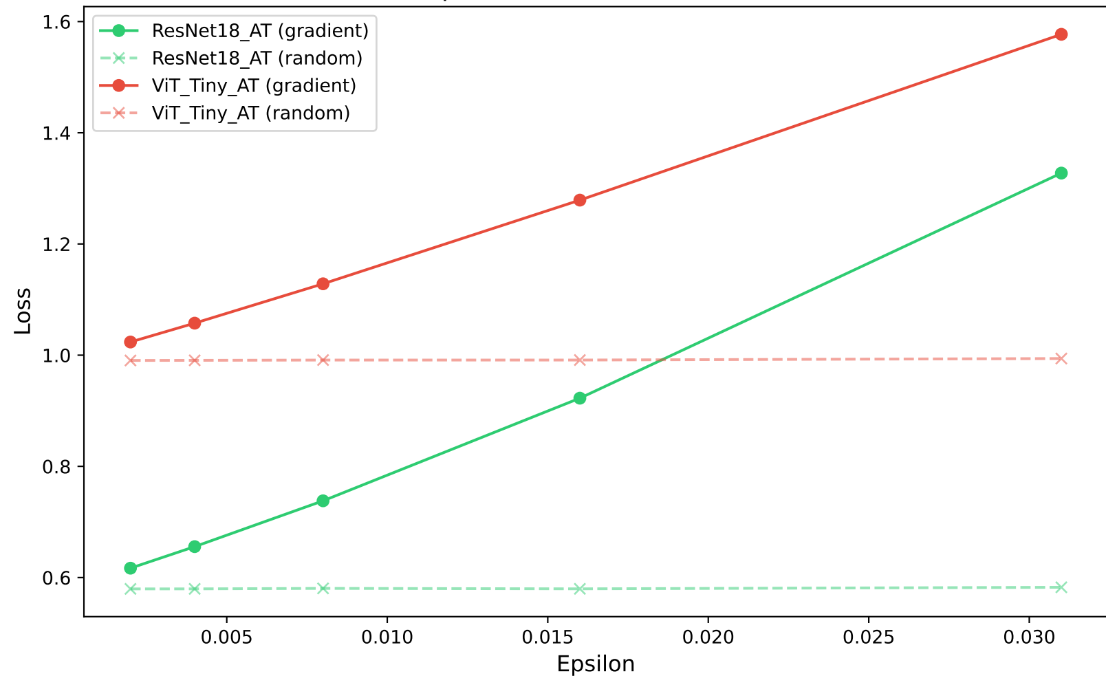
Loss Landscape: Gradient vs Random Perturbation
