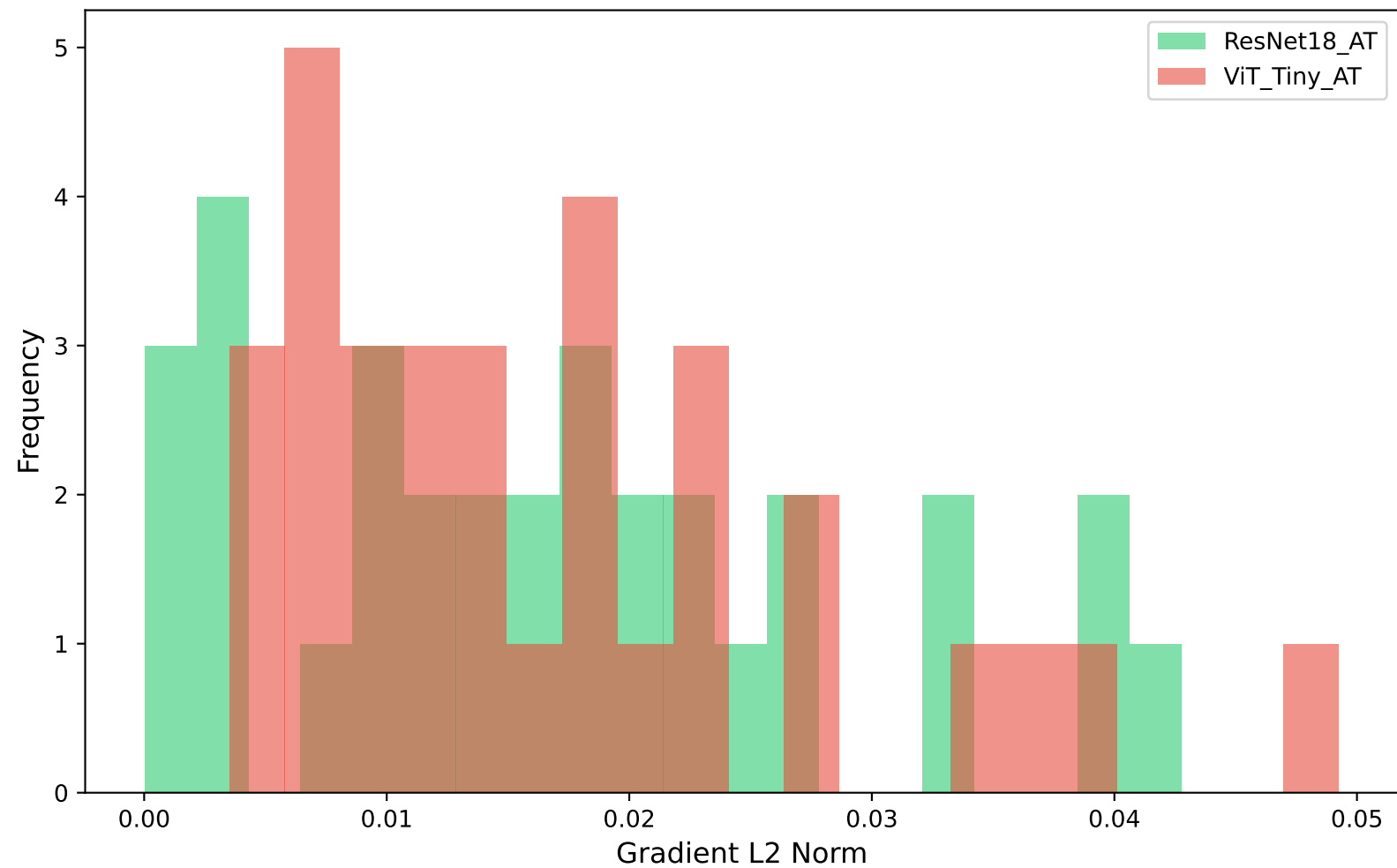
Gradient Norm Distribution: CNN vs ViT
