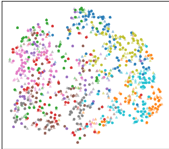
ViT-Tiny (AT)
