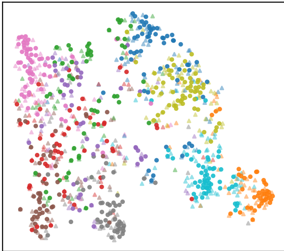
ResNet-18 (AT)
