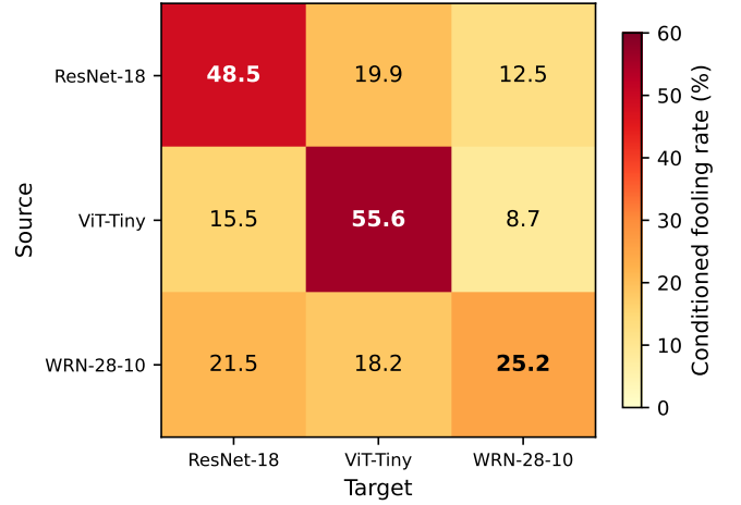
Fig. 4: Conditioned (target-correct) transfer fooling rates, mean over three seed pairs. Off-diagonal asymmetry under this protocol is +4.4 points; Table III shows how far the same quantity moves under other protocols.
