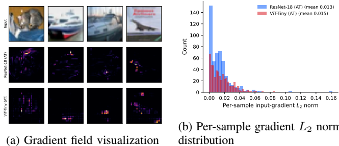
Fig. 5: Gradient characteristics comparison. (a) Input-gradient magnitude maps for representative test images with the corresponding PGD-10 perturbations. (b) Distribution of per-sample gradient L_2 norms for both architectures.
