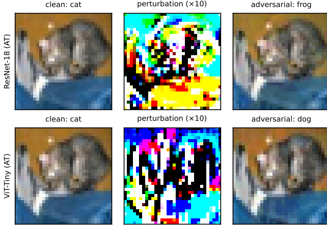
Fig. 3: For each model, its own white-box PGD-10 attack on the same test image, showing the clean prediction, the perturbation magnified 10\times , and the adversarial prediction. Perturbations are bounded by \epsilon=8/255 and remain visually subtle at this scale.
