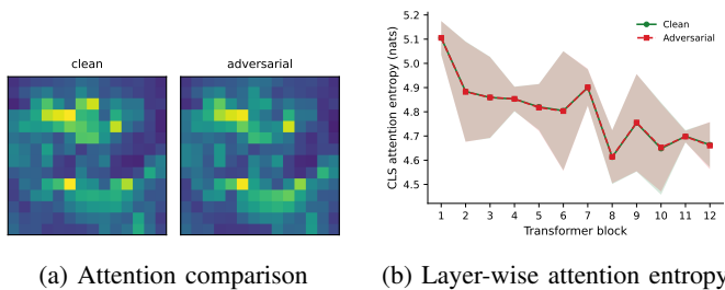
Fig. 8: ViT attention analysis under attack: (a) clean vs. adversarial CLS attention for a representative sample; (b) per-layer entropy of the CLS attention distribution for clean and adversarial inputs.
