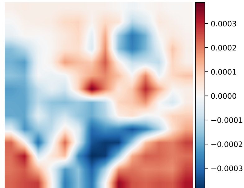
Layer 6 Difference
