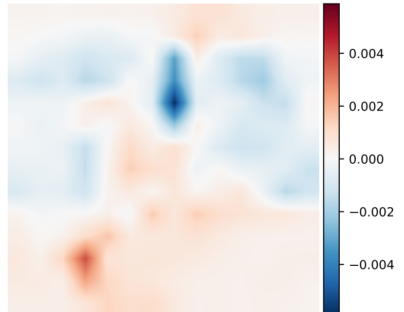
Layer 12 Difference
