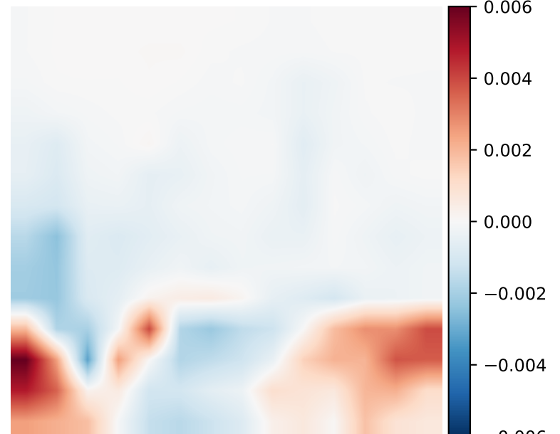
Layer 12 Difference
