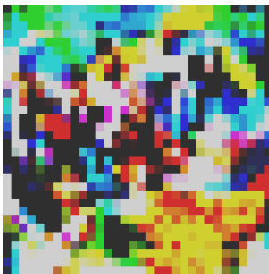
Perturbation ( \times 10 )
