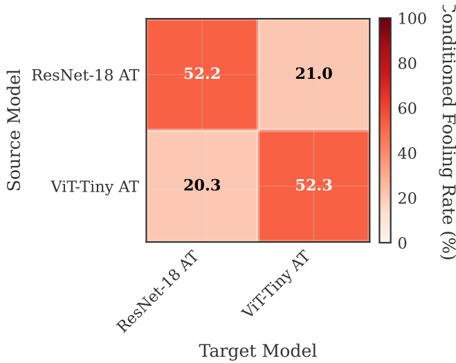
Fig. 4: Conditioned transfer fooling-rate heatmap ( n=10,000 ). Off-diagonal transfer is symmetric once target clean error is controlled for (21.0% vs 20.3%).
