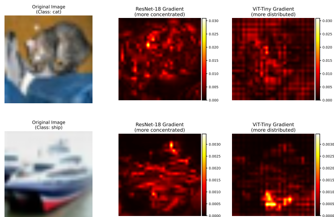
Fig. 5: Gradient characteristics comparison. (a) Input-gradient magnitude maps for representative test images with the corresponding PGD-10 perturbations. (b) Distribution of per-sample gradient L_2 norms for both architectures.
