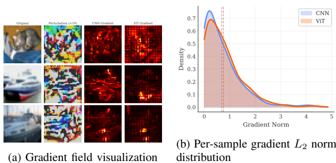
Fig. 5: Gradient characteristics comparison. (a) Input-gradient magnitude maps for representative test images with the corresponding PGD-10 perturbations. (b) Distribution of per-sample gradient L_2 norms for both architectures.
