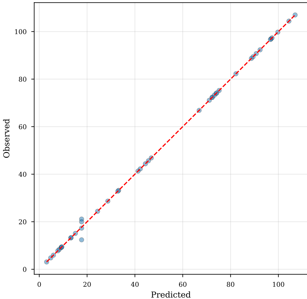
Calibration: Toughness
