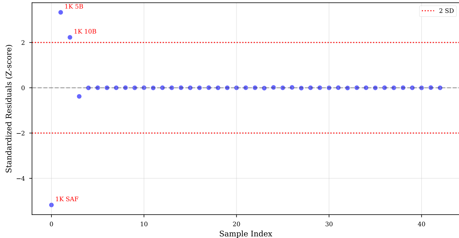
Toughness: Residuals by Sample ID
