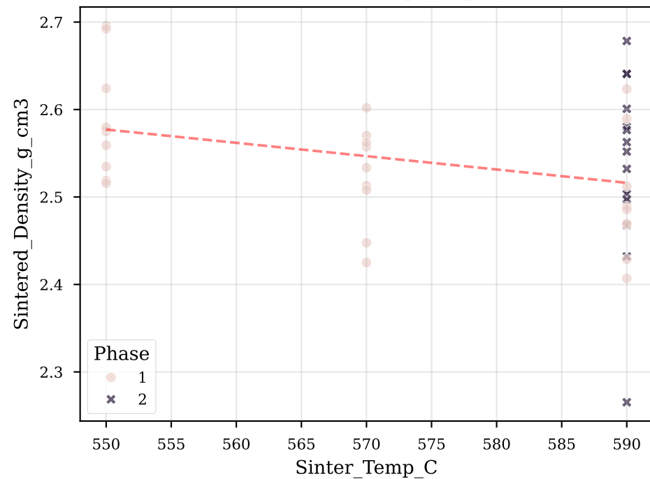
Density vs Sinter_Temp_C
